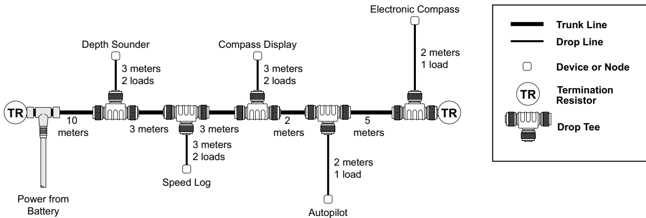
FIGURE 6. End-Powered Network
